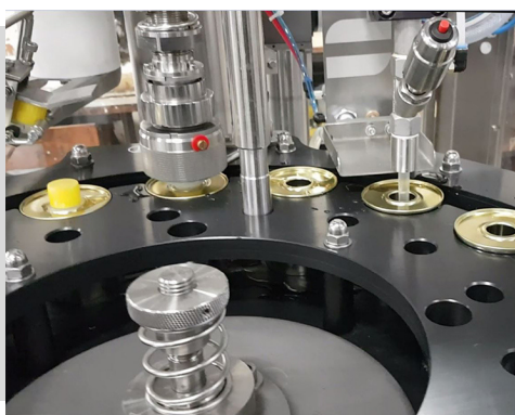
1 filling head and 1 capping head monobloc
