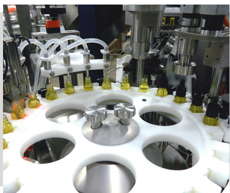
4 filling heads and 2 screwing heads monobloc
