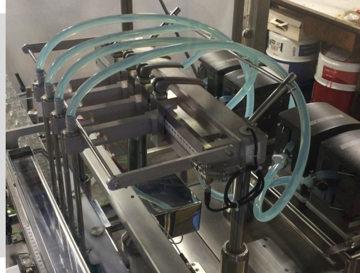
Peristaltic dosing circuit
