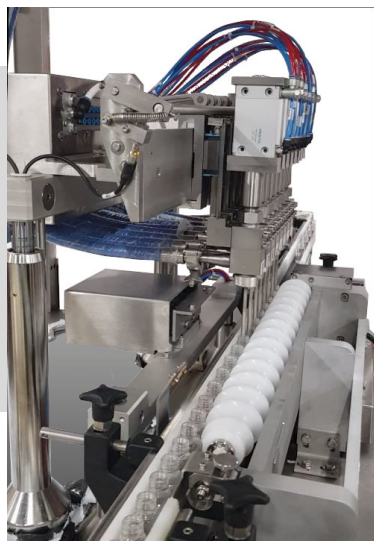
Worm gear for bottles (option)
